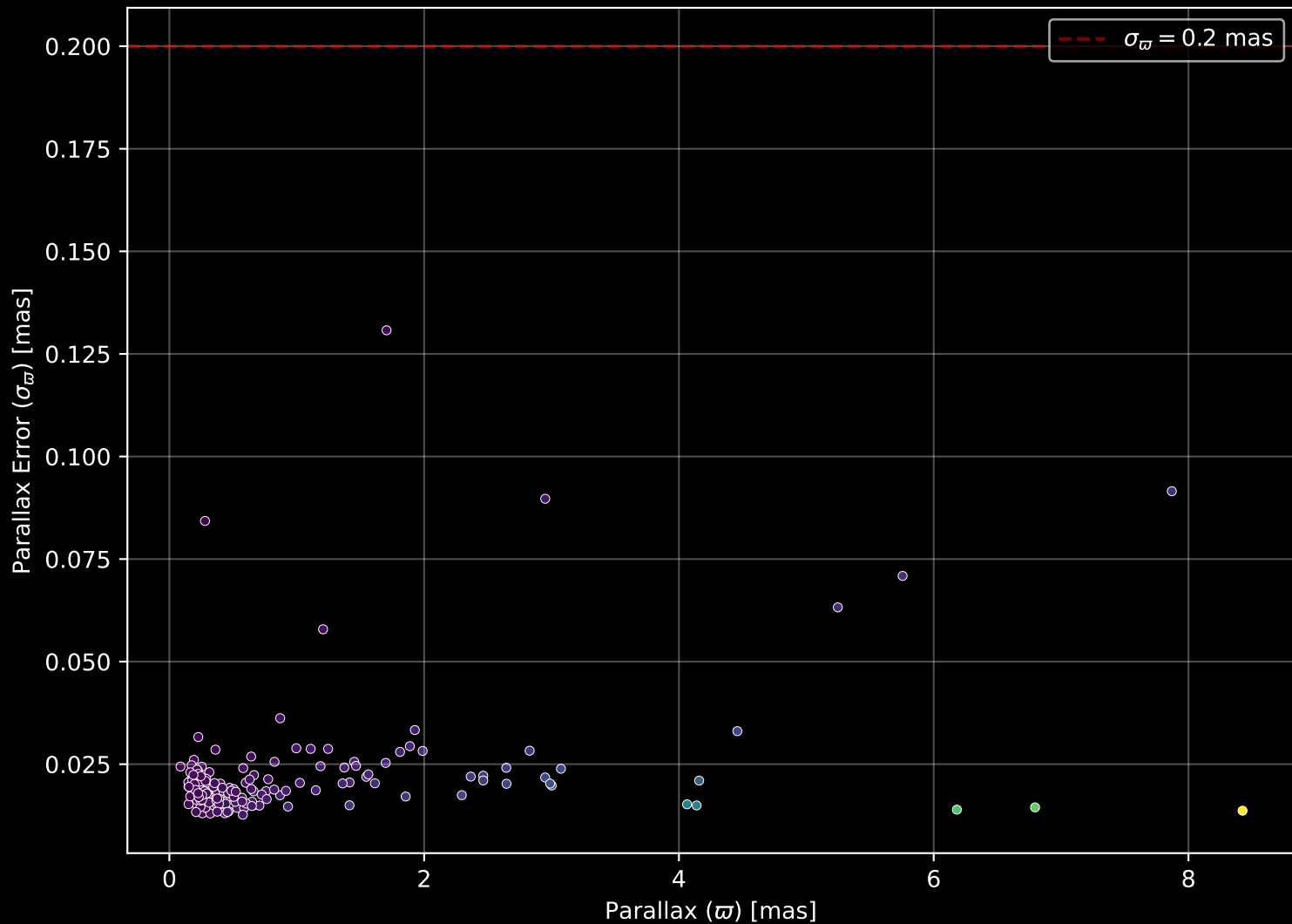
APOGEE DR17 Field: [188+12] Parallax Quality (n= 182)
