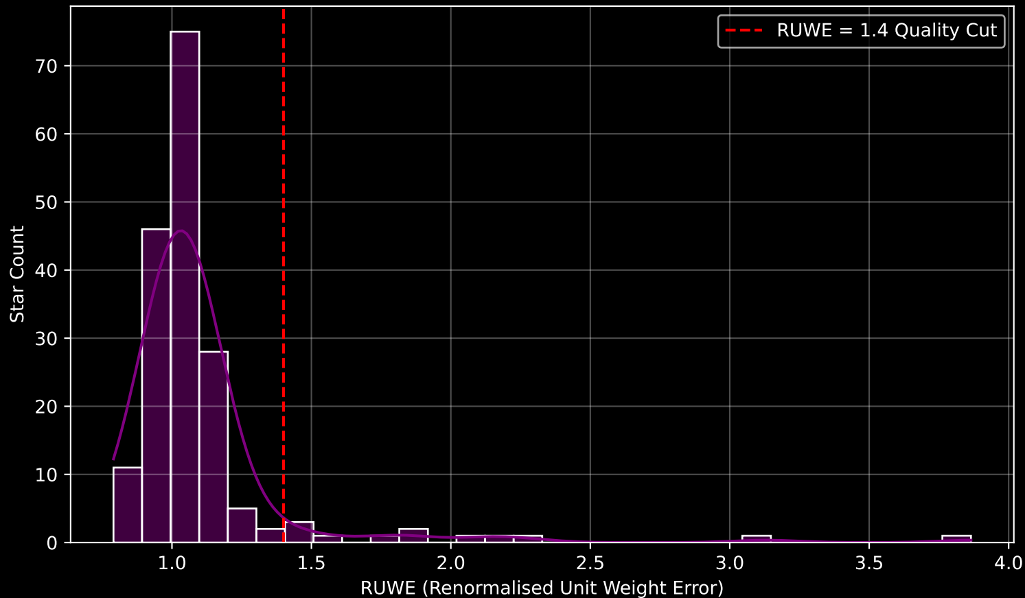
GAPOGEE DR17 Field [188+12] RUWE Distribution (n= 179)
