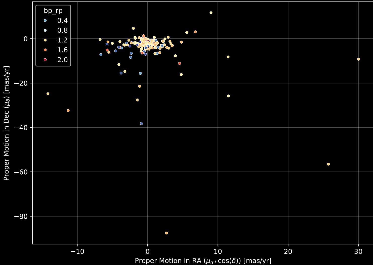
APOGEE DR17 Field: [188+12] Proper Motion Diagram (n= 182)
