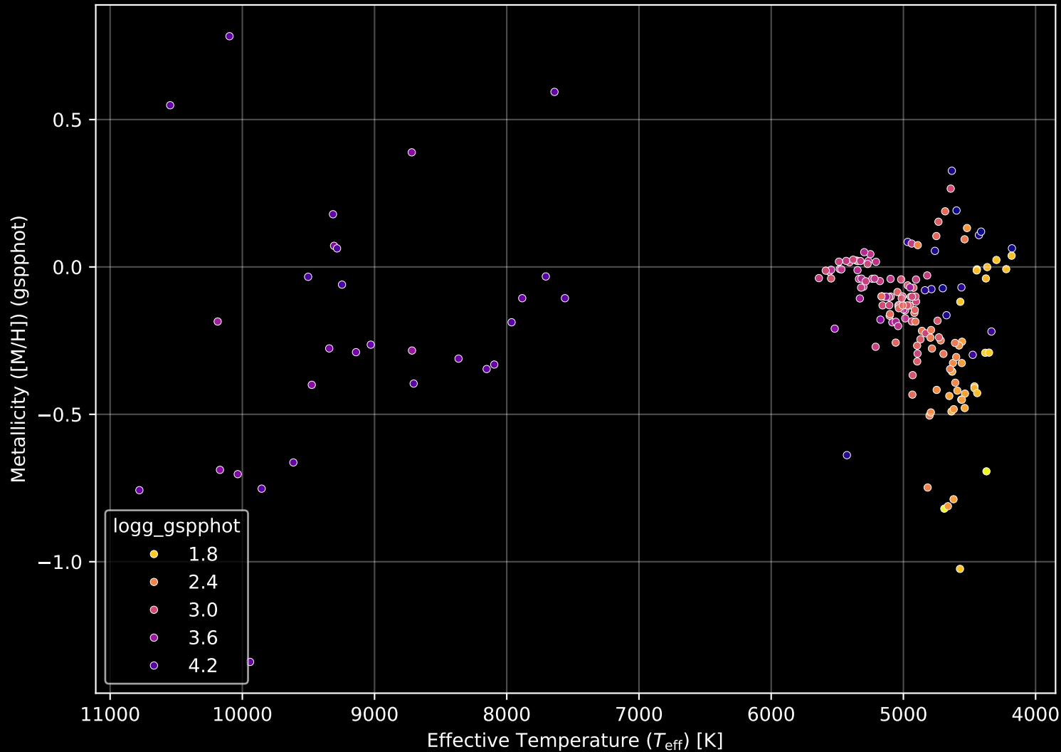
APOGEE DR17 Field: [188+12] Stellar Population Parameters (n= 182)
