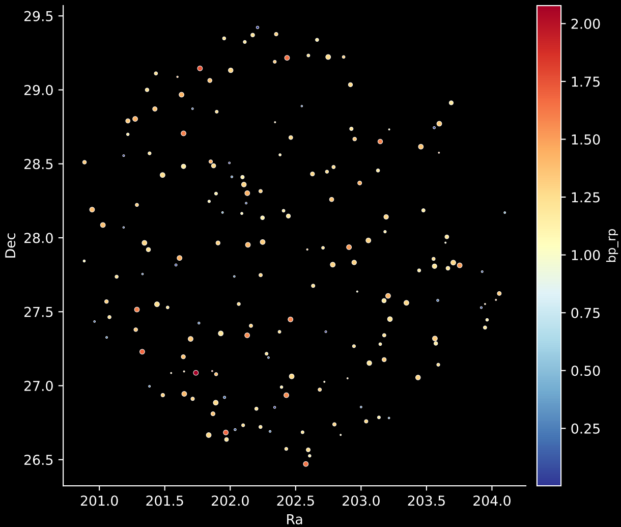
APOGEE DR17 Field: [188+12] Stars: 182
