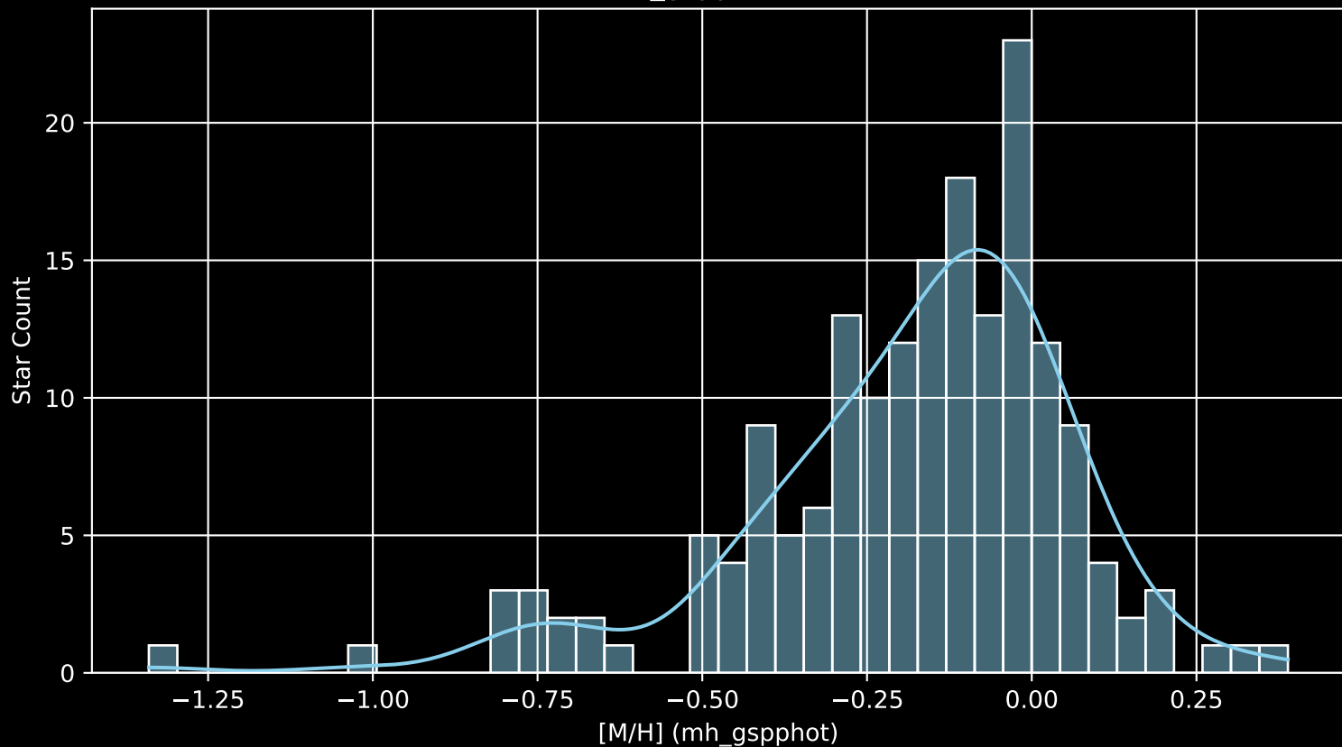
APOGEE DR17 Field: [188+12 [M/H] (mh_gspphot) (n= 179)
